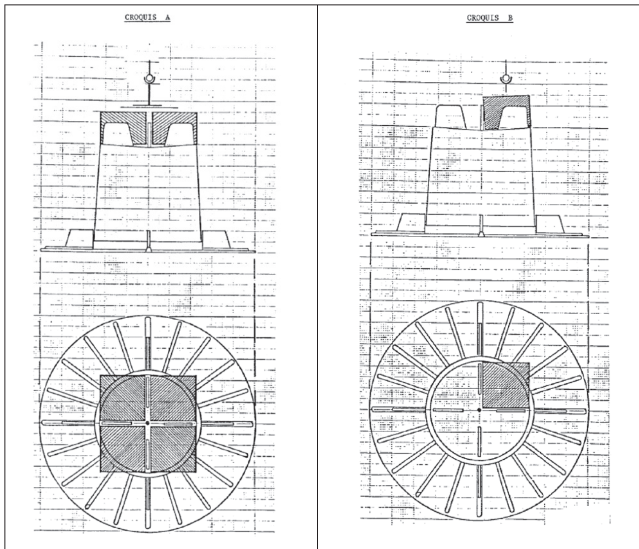
Figure B2 – Application de la charge
