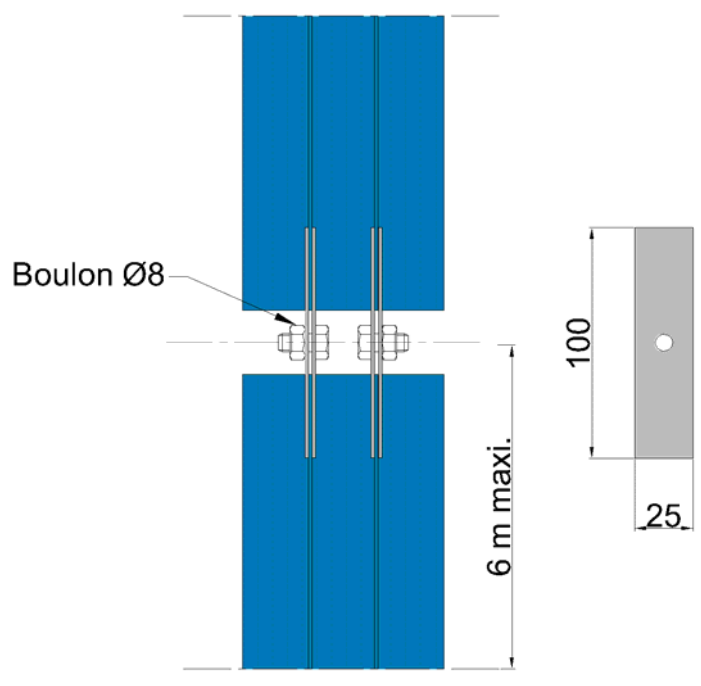
Figure 12 – Aboutement
