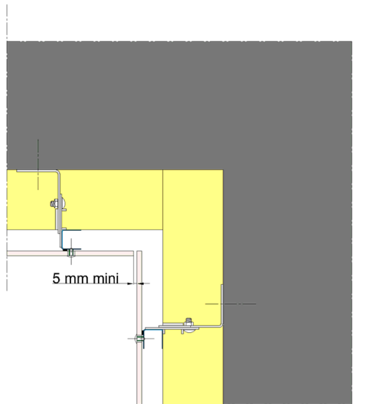
Figure 20 - Angle rentrant
