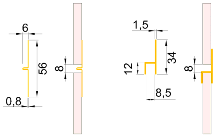
Joint Aluminium
