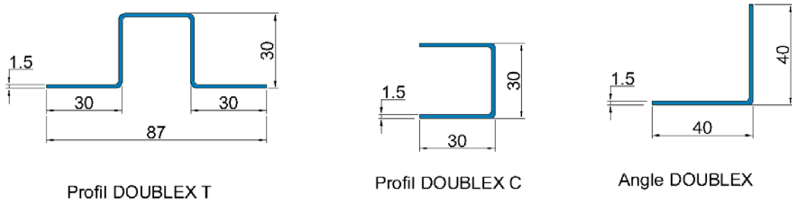
Figure 4 - Profils DOUBLEX
